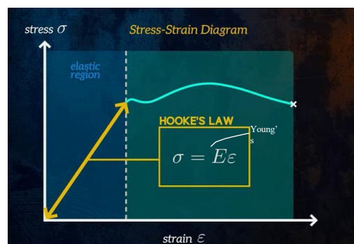
Gambar 2. 4 Diagram Tegangan-Regangan
