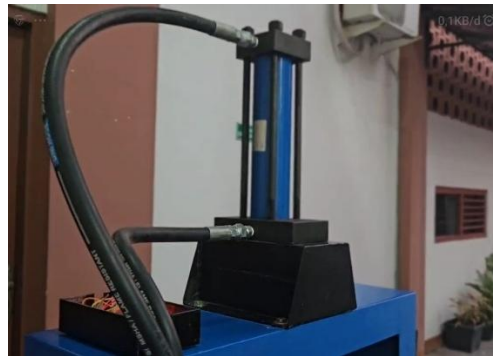
Gambar 3. 14 Flexible hose
