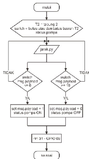
Gambar 6. Flowchart Sistem Monitoring Ketinggian Air
