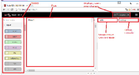
Gambar 2 Tampilan Node-RED
