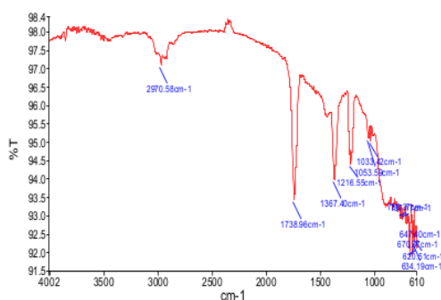
Fig. 1. FTIR Polyvinyl Alcohol Spectrum (PVA)
