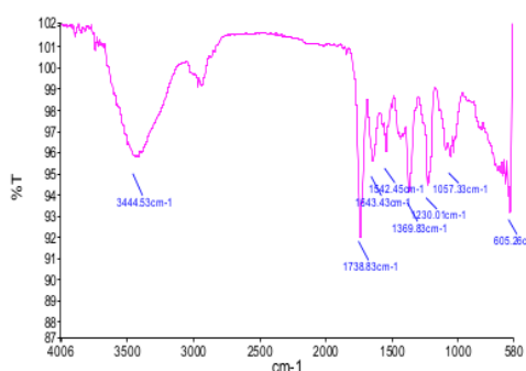
Fig. 6. FTIR Spectrum PVA-Collagen 1% + Chitosan 2%
