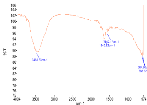
Fig. 3. PVA-Collagen Spectrum 0.8%
