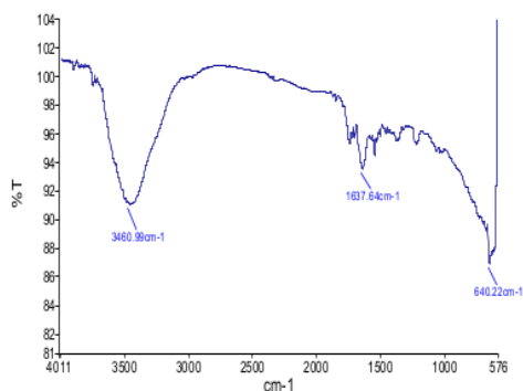
Fig. 5. FTIR Spectrum PVA-Collagen 0.8% + Chitosan 2%
