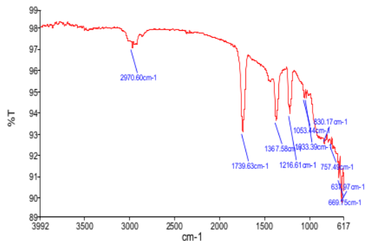
Fig. 2. 2% FTIR PVA-Chitosan spectrum
