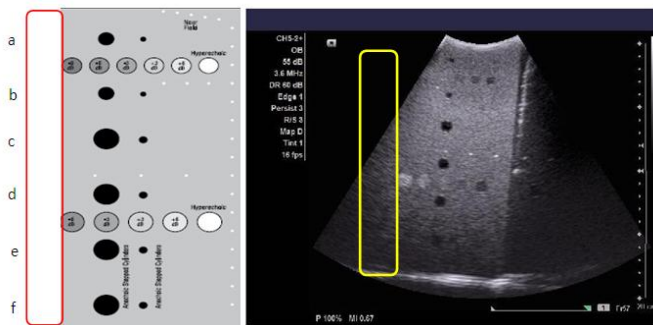
Figure 1. The objects in ultrasound phantom, objects (a, b, c, d, e, f) in the red column are original anechoic stepped cylinder from phantom, while the image of the ultrasound scanning, anechoic stepped cylinder are shown the yellow column.
