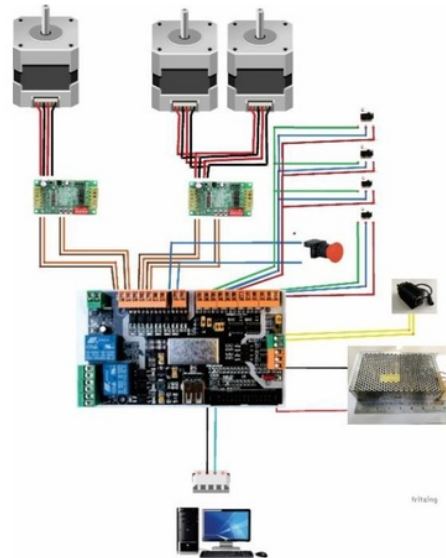
Gambar 5. Wiring diagram mesin CNC laser engraving .
